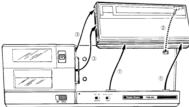
Figure 4. Computer-Interface Alignment
